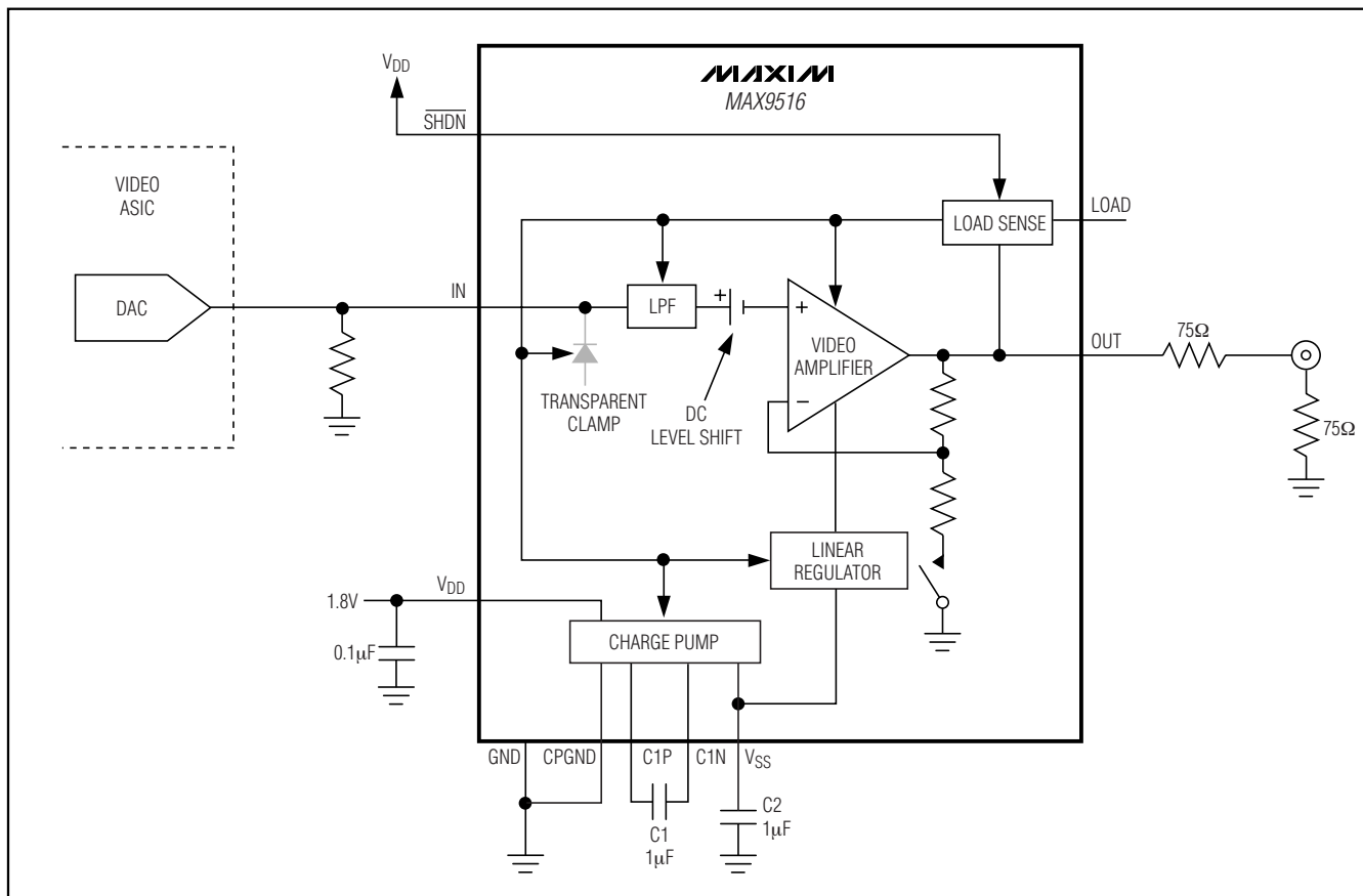
Figure 7. DC-Coupled Input
