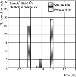
Operate and Release Time Distribution (See note.)
