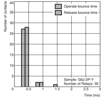
Operate and Release Bounce Time Distribution (See note.)
