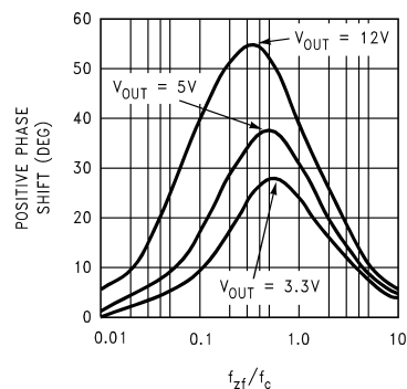
Phase Lead Provided by C_F
