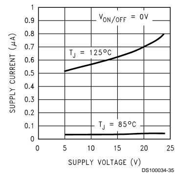
Leakage Current
