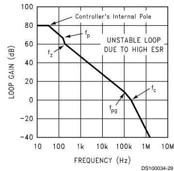
High ESR Unstable without Feed-Forward
