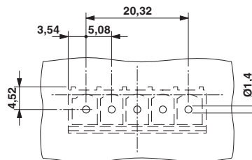
Drilling diagram
