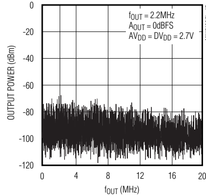
FFT PLOT, DAC2 ( f_{CLK} = 40MHz , 2048-POINT DATA RECORD)
