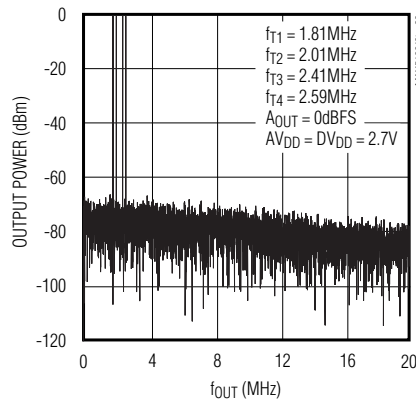
MTPR PLOT ( f_{CLK} = 40MHz , 4096-POINT DATA RECORD)
