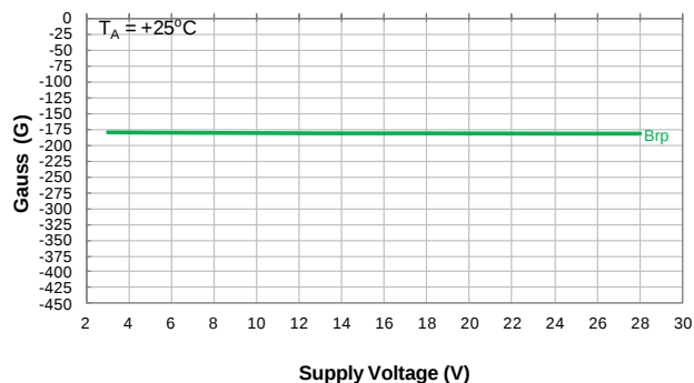
Switch Release Point B_{rp} vs Supply Voltage
