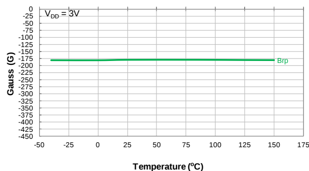
Switch Release Point B_{rp} vs Temperature
