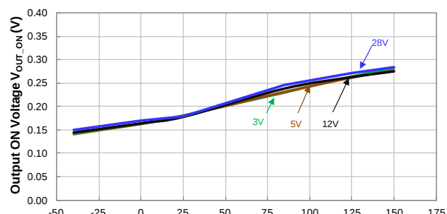
Temperature ( ^\circ\text{C} ) Output ON Voltage vs Temperature
