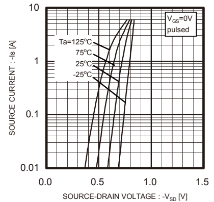
Fig.6 Source-Current vs. Source-Drain Voltage
