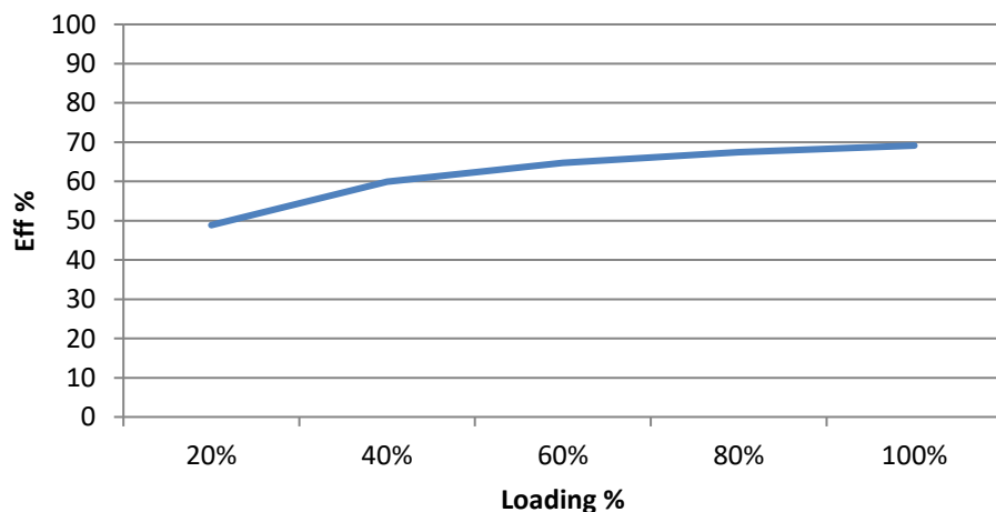
AM1DR-2405SZ Efficiency vs. Loading
