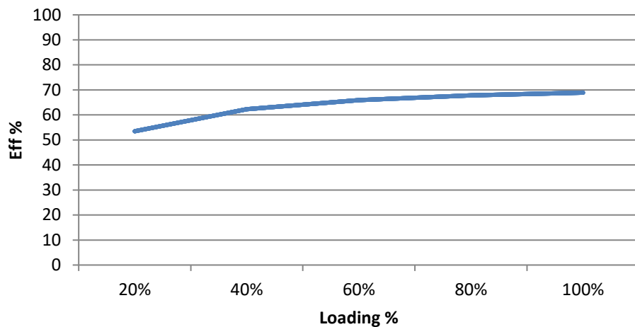
AM1DR-0505SZ Efficiency vs. Loading
