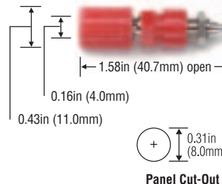
Panel Cut-Out
