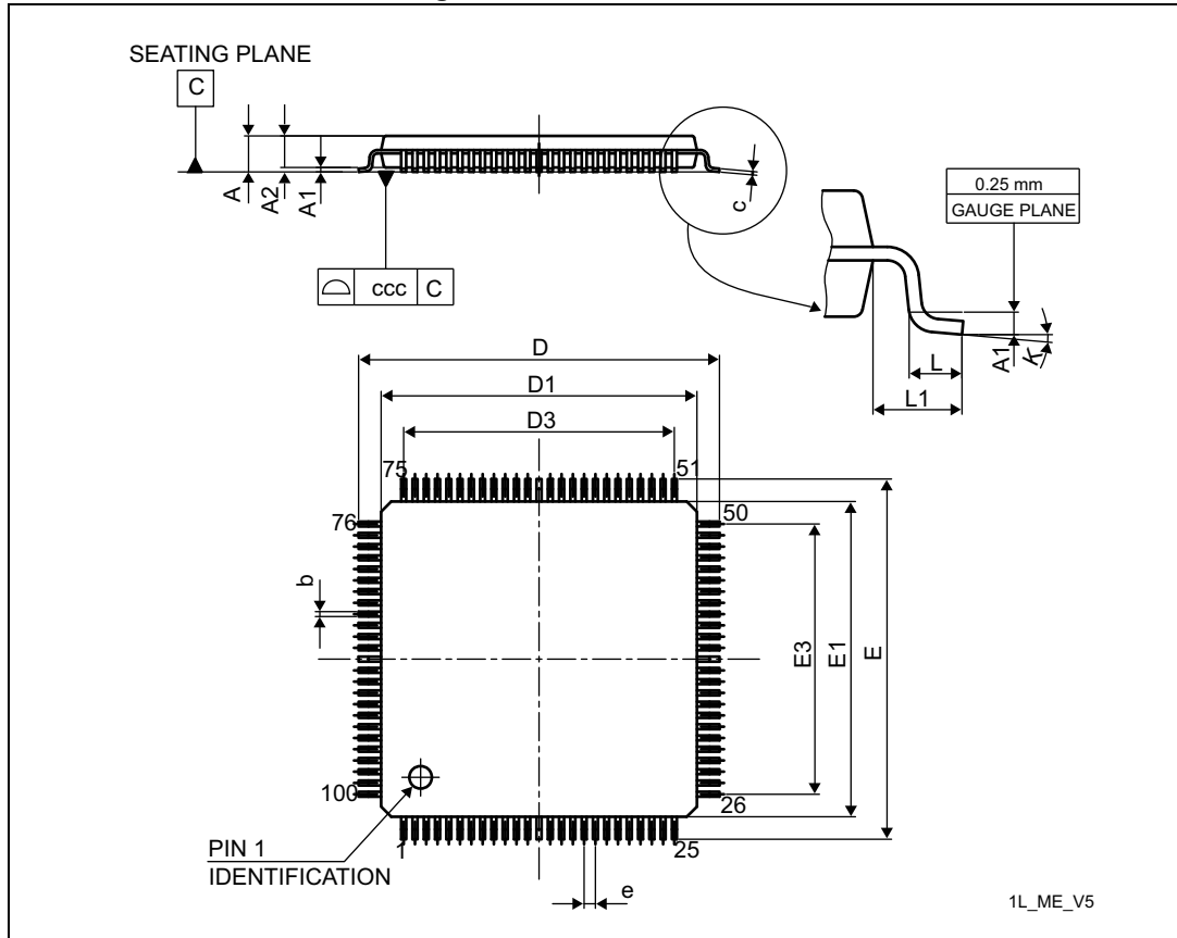
Figure 85. LQFP100 outline
