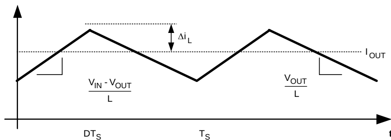
Figure 23. Inductor Current
