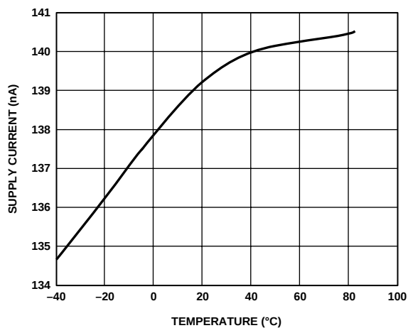
Figure 8. Power-Down Supply Current vs. Temperature
