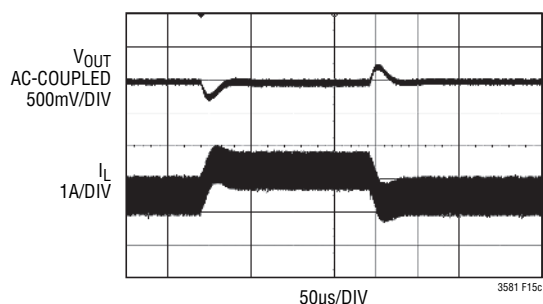
Figure 15c. Transient Response is Well Damped
