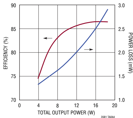
Efficiency and Power Loss at V_{IN} = 12V
