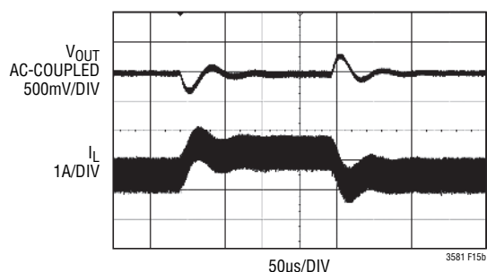
Figure 15b. Transient Response is Better
