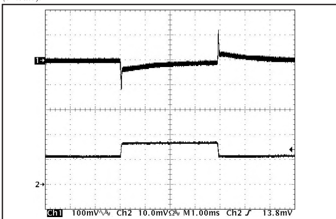
Figure 11: Output voltage response to step-change in load current (50%-75%-50% of I_{out(max)} ; dI/dt = 0.1A/\mu s ). Load cap: 10 \mu F, 100 m \Omega ESR tantalum cap and 1 \mu F ceramic cap. Ch 1: V_{out} (100mV/div), Ch 2: I_{out} (20A/div).
