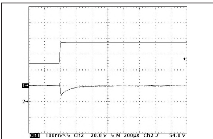
Figure 17: Output voltage response to step-change in input voltage (48V to 75V), at 45A load current. Load cap: 10 \mu F tantalum capacitor and 1 \mu F ceramic cap. Ch 1: V_{out} (100mV/div), Ch 2: V_{in} (20V/div).
