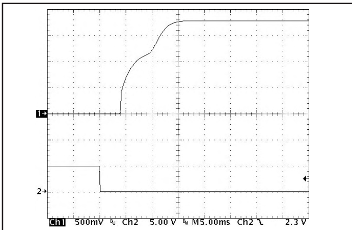
Figure 9: Turn-on transient at full load (resistive load) (5 ms/div). Load cap: 10 \mu F, 100 m \Omega ESR tantalum capacitor and 1 \mu F ceramic capacitor. Input voltage pre-applied. Ch 1: V_{out} (500 mV/div), Ch 2: ON/OFF input (5 V/div).
