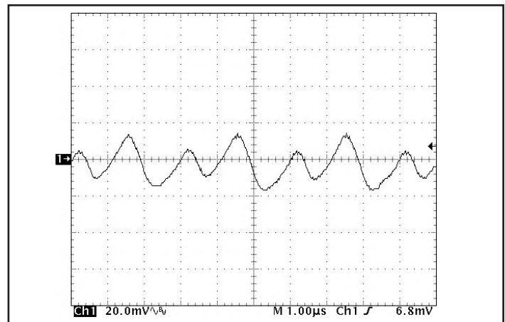
Figure 16: Output voltage ripple at nominal input voltage and rated load current (20 mV/div). Load capacitance: 1 \mu F ceramic capacitor and 15 \mu F tantalum capacitor. Bandwidth: 20 MHz. See Figure 13.
