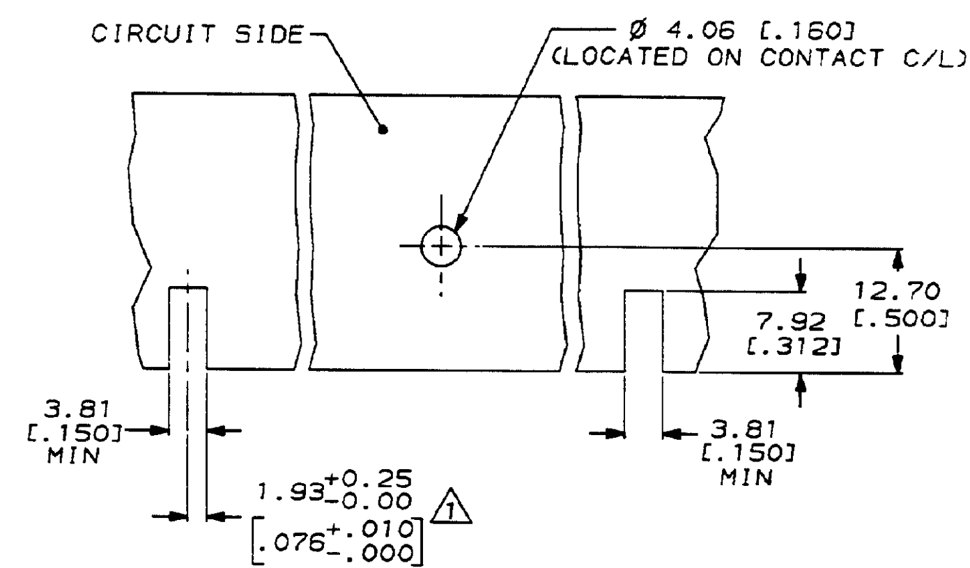
RECOMMENDED LAYOUT FOR P.C. BOARD SCALE 2:1
