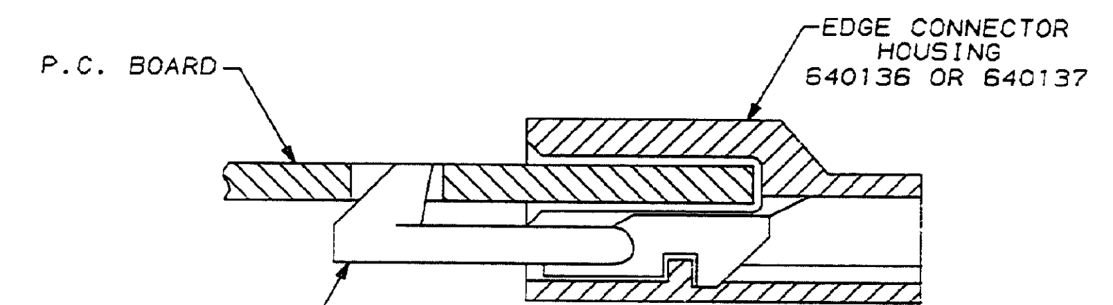
PROFILE VIEW SCALE 5:1
