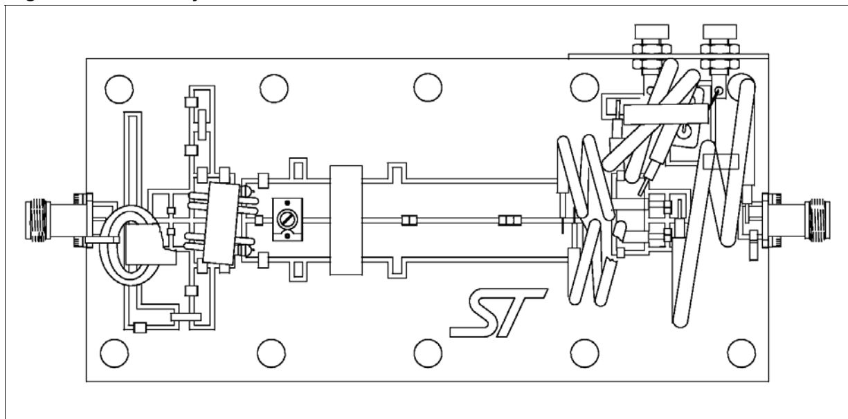
Figure 10. Circuit layout
