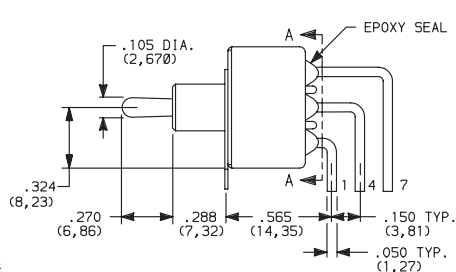
Actuator Shown In Pos. 1 Terminals & Support
