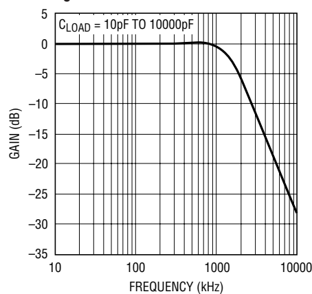
V_{OCM} Gain vs Frequency, V_S = \pm 2.5V
