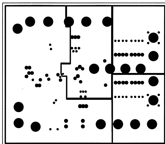
Figure 28. Internal Plane 2
