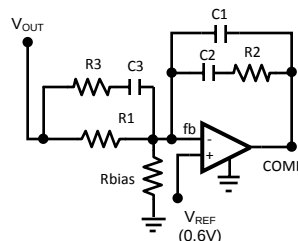
Figure 23. Type 3 Compensation
