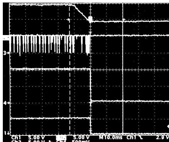
CH1: PGOOD, CH2: VIN, CH3: LDRV, CH4: V 0 Output 1V @ 0.02A, VIN = 9.75V, FPWM, L = 10μH, f = 300kHz, C OUT = 660μF
