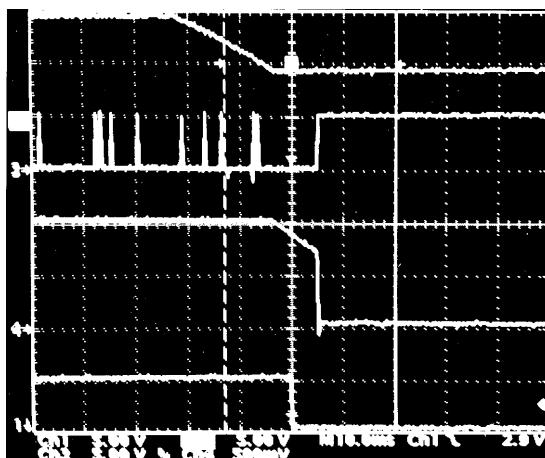
CH1: PGOOD, CH2: VIN, CH3: LDRV, CH4: V 0 Output 1V @ 0.02A, VIN = 9.75V, SKIP, L = 10μH, f = 300kHz, C OUT = 660μF
