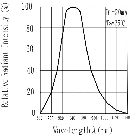
Fig. 2 Spectral Distribution
