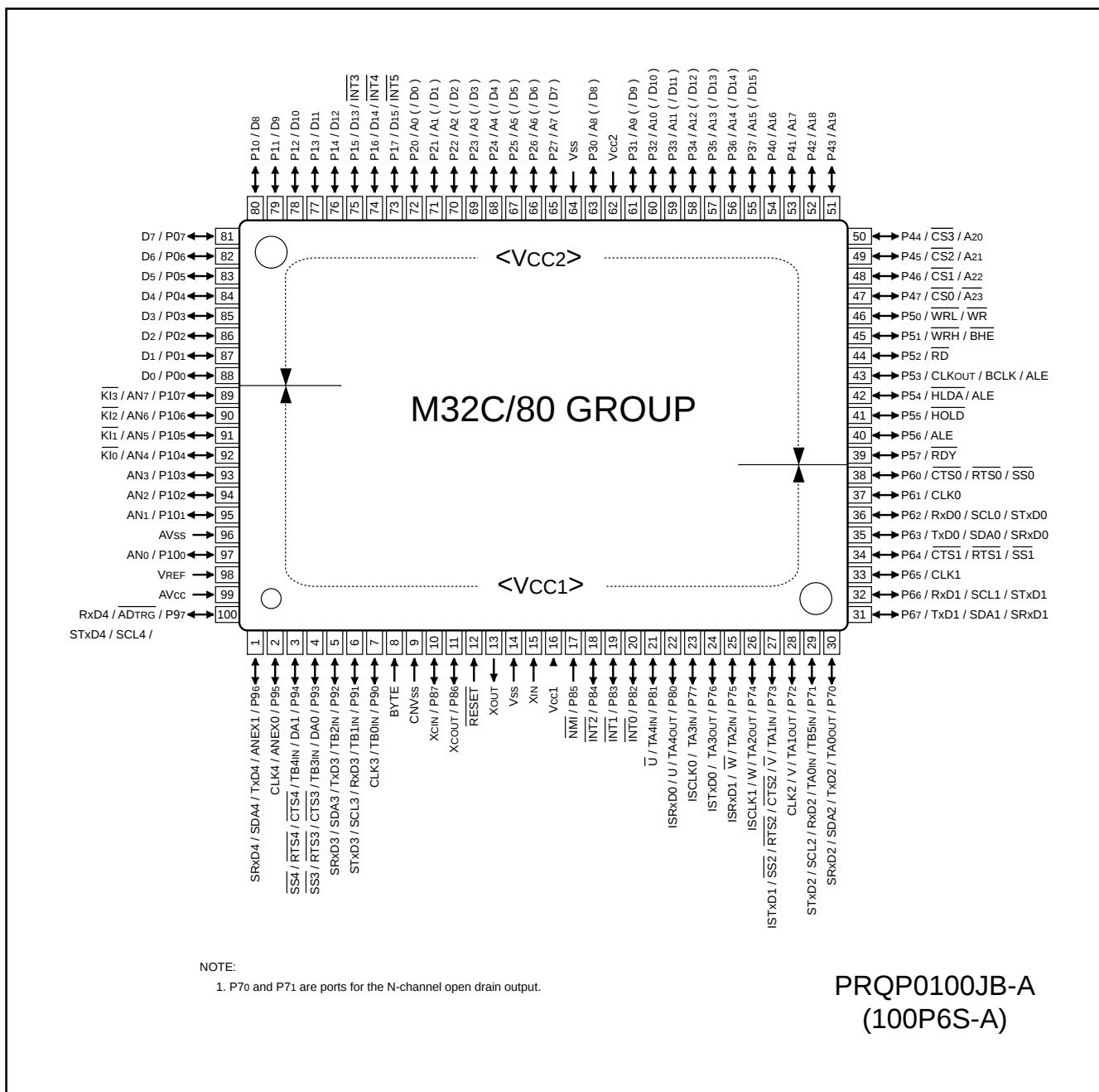
Figure 1.3 Pin Assignment
