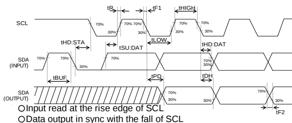
Figure 1.-(a). Serial Input / Output Timing
