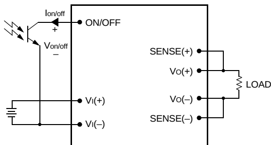
Figure 15. Remote On/Off Implementation Lineage Power
