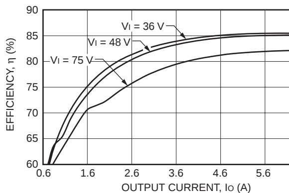
Figure 4. Typical QW075B1 Efficiency vs. Output Current at Room Temperature
