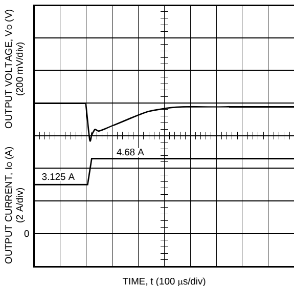
Figure 9. Typical QW050B1 Transient Response to Step Increase in Load from 50% to 75% of Full Load at Room Temperature and 48 Vdc Input (Waveform Averaged to Eliminate Ripple Component.)
