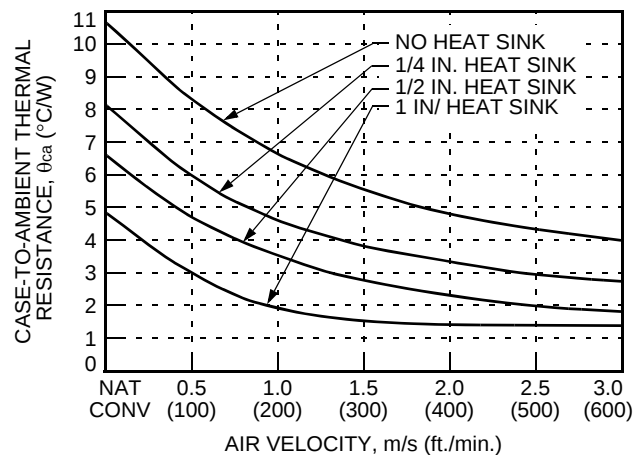
Figure 24. Case-to-Ambient Thermal Resistance Curves; Longitudinal Orientation
