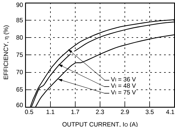
Figure 3. Typical QW050B1 Efficiency vs. Output Current at Room Temperature
