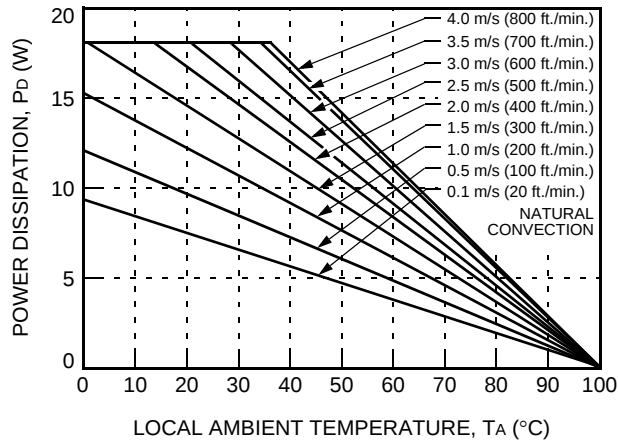
Figure 22. Forced Convection Power Derating with No Heat Sink; Either Orientation
