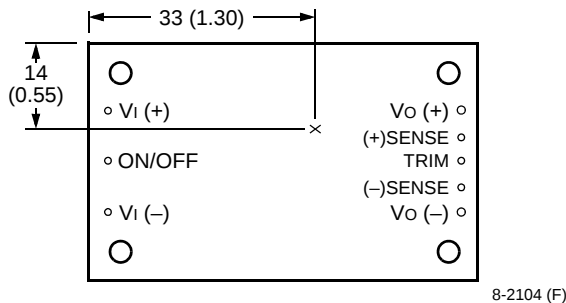
Figure 19. Case Temperature Measurement Location
