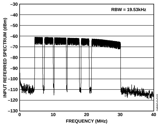
Figure 10. Spectral Plot with 4K FFT of 111-Carrier DMT Signal with PAR = 11 dB, P_{\text{IN}} = -33.7 dBm, LPF's f_{-3\text{dB}} = 32 MHz and RxPGA = 36 dB
