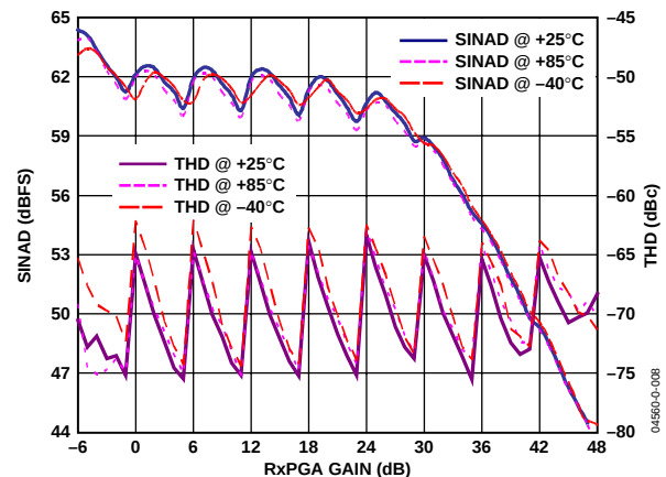
Figure 8. SINAD/THD Performance vs. RxPGA Gain and Temperature ( f_{\text{IN}} = 5 MHz)
