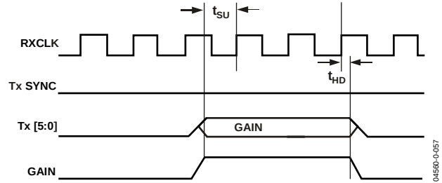
Figure 57. Updating RxPGA via Tx[5:0] in Full-Duplex Mode
