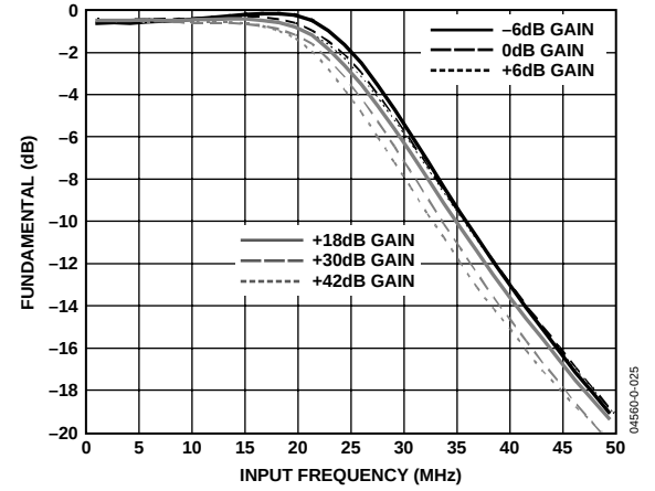
Figure 25. Rx Low-Pass Filter Amplitude Response vs. RxPGA Gain (LPF's f_{-3\text{ dB}} = 33\text{ MHz} )
