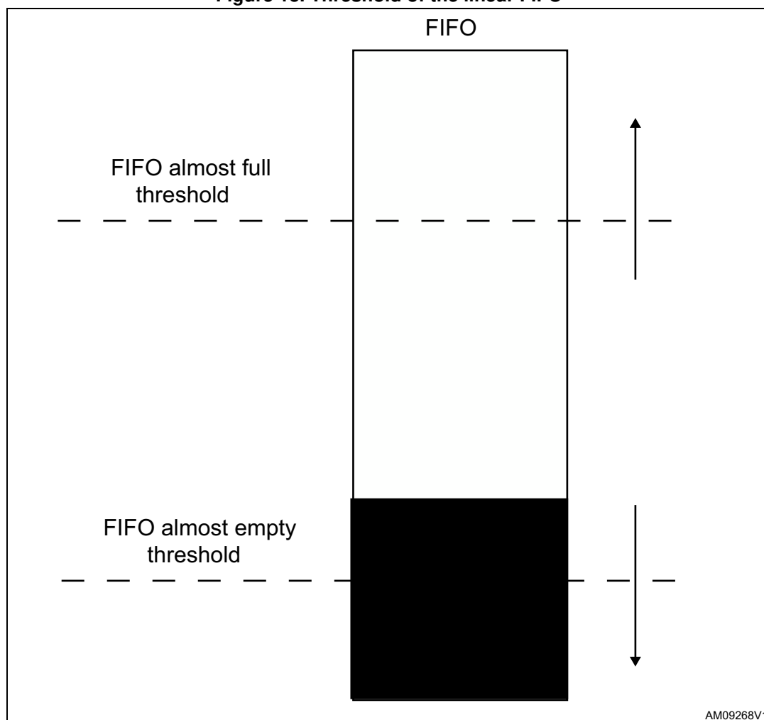
Figure 13. Threshold of the linear FIFO
