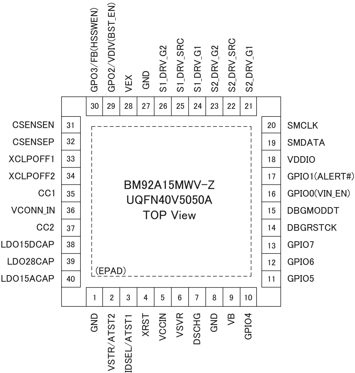
Figure 1-1 Pin configuration
