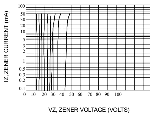
Fig. 7-VZ = 12 THRU 40 VOLTS
