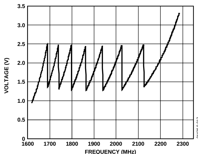
Figure 14. Frequency vs. V_{TUNE} , ADF4360-2
