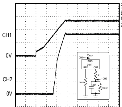
STARTUP DELAY (V BIAS = 2.7V, I REF = 2.5mA)
