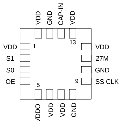
16-pin QFN
