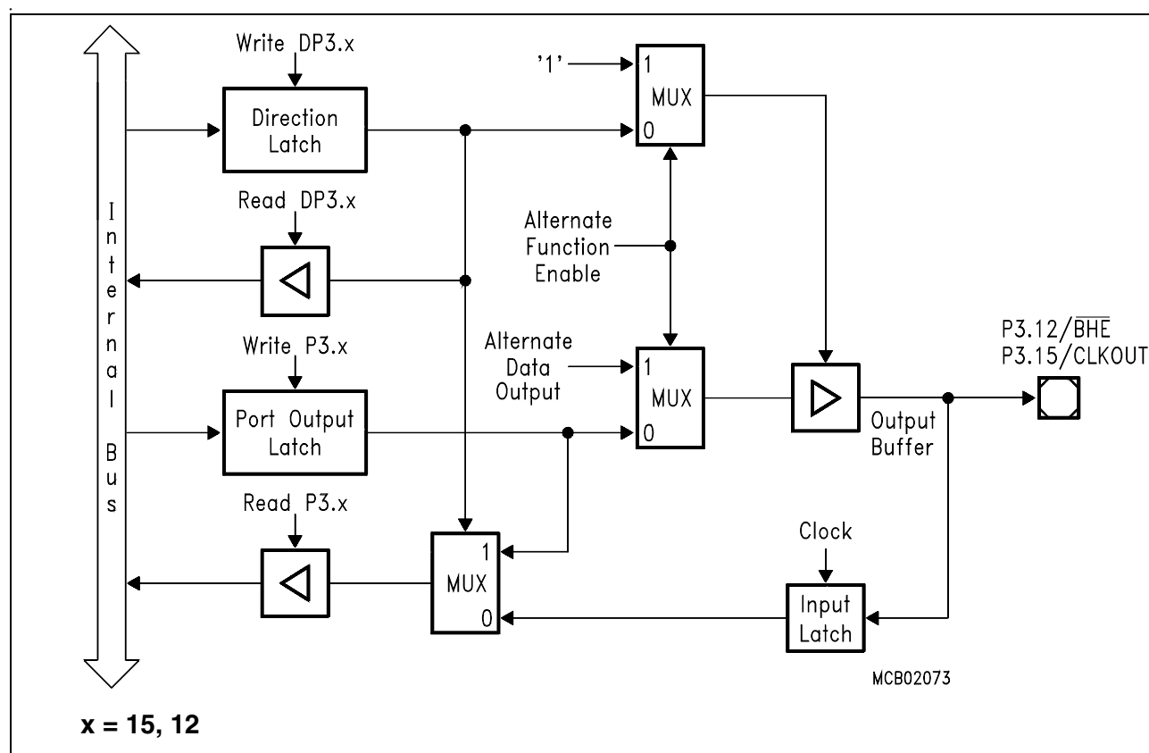
Figure 9-8 Block Diagram of Pins P3.15 (CLKOUT) and P3.12 ( \overline{\text{BHE}}/\overline{\text{WRH}} )
