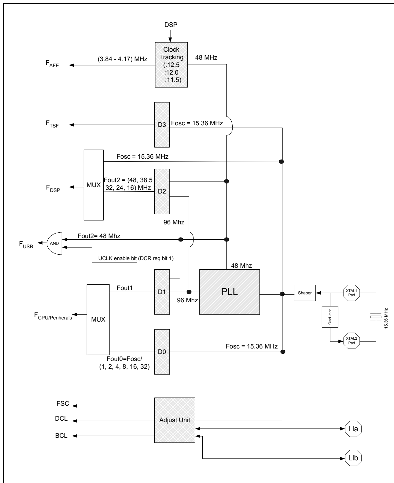
Figure 4-1 Clock Concept
