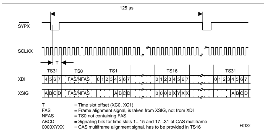
Figure 24 2.048 MHz Transmit Signaling Highway (E1)
