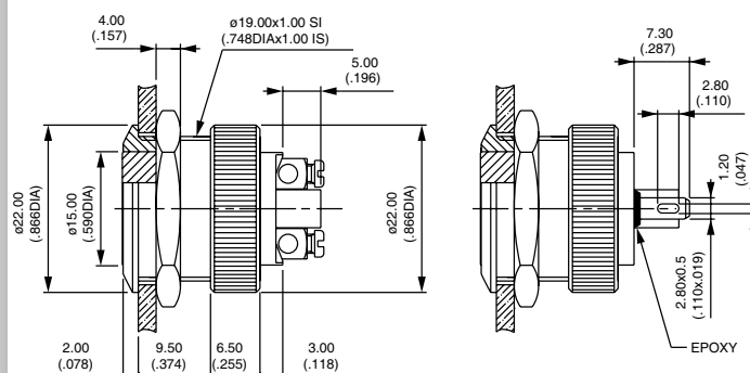
Hex nut 22 (.866) across flats
