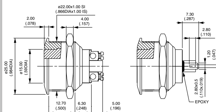
Hex nut 25 (.984) across flats
