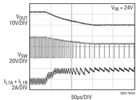
Frequency Foldback Waveforms When Output Short-Circuit
