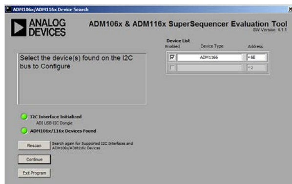
Figure 8. Device Search
