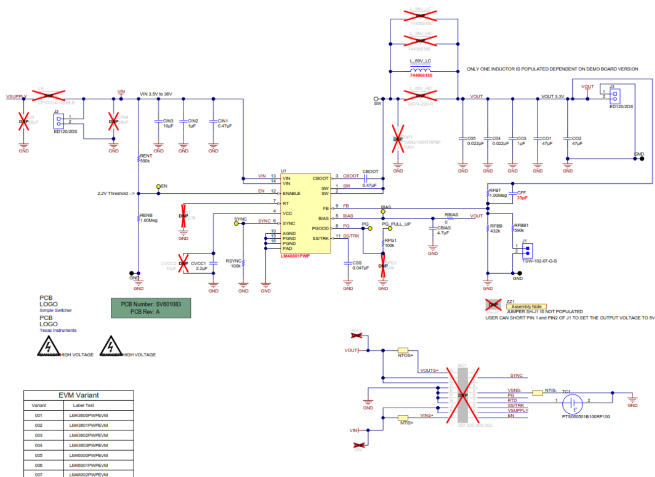
Figure 2. LM46001EVM Schematic
