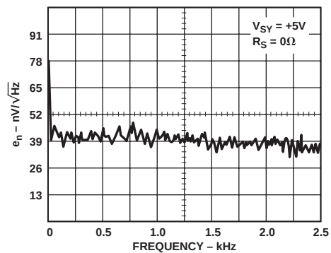
Figure 36. Voltage Noise Density at +5 V from 0 Hz to 2.5 kHz
