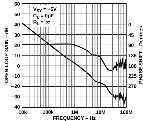
Figure 12. Open-Loop Gain and Phase Shift vs. Frequency at +5 V
