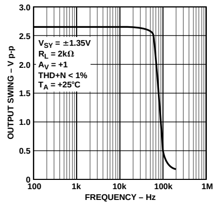
Figure 30. Maximum Output Swing vs. Frequency at +2.7 V
