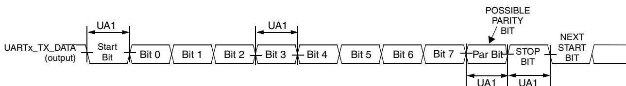
Figure 94. UART RS-232 Serial Mode Transmit Timing Diagram
