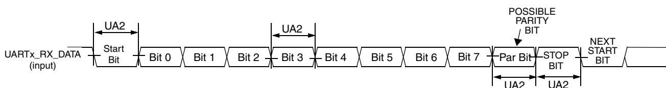
Figure 95. UART RS-232 Serial Mode Receive Timing Diagram
