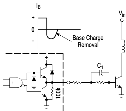
Figure 24. Bipolar Transistor Drive
