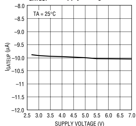
I_{\text{GATEUP}} vs Supply Voltage
