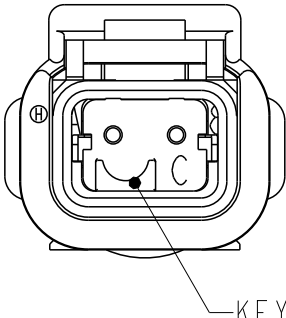
DTMH04-2PC -C- KEY TPA COLOR: GREEN
