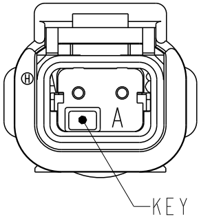
DTMH04-2PA -A- KEY TPA COLOR: GREY
