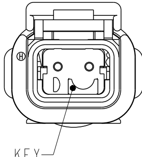
DTMH04-2PD -D- KEY TPA COLOR: BROWN
