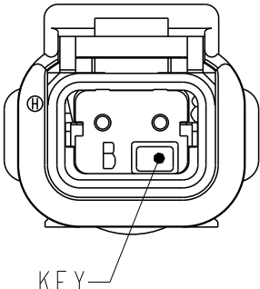
DTMH04-2PB -B- KEY TPA COLOR: BLACK
