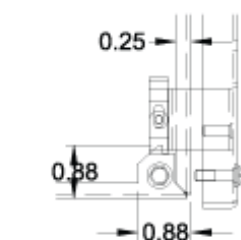
Hinge Detail
