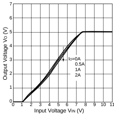
Rise Characteristics(SI-3052P)
