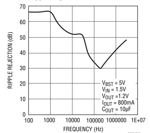
Ripple Rejection
