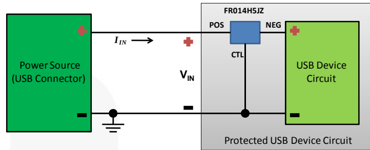
Figure 2. Typical Schematic
