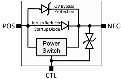
Figure 1. Block Diagram
