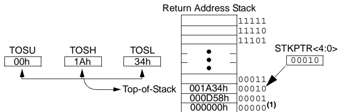
FIGURE 4-5: RETURN ADDRESS STACK AND ASSOCIATED REGISTERS
