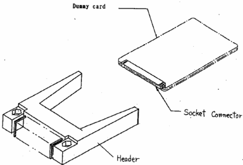
Fig. 5.1 Construction
