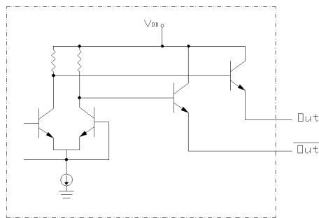
Figure 7. Standard PECL Output Configuration
