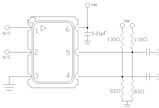
Figure 9. Pull-Up Pull Down Termination
