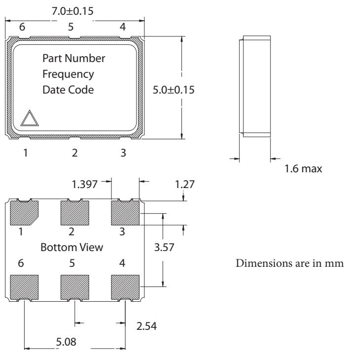
Figure 4. Package A Outline Drawing
