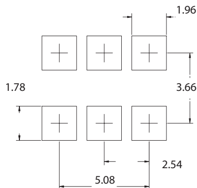
Figure 5. Optional Package Outline Drawing
