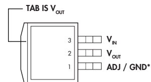
DD PACKAGE (Top View)
