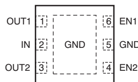
TPS718xx, TPS719xx DRV Package 2mm x 2mm SON-6 (Top View)
